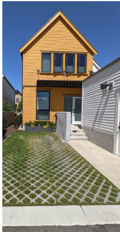
Example of a pervious driveway treatment to allow for rainwater infiltration (guideline 37).
